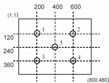
Fig.1 Measuring point
