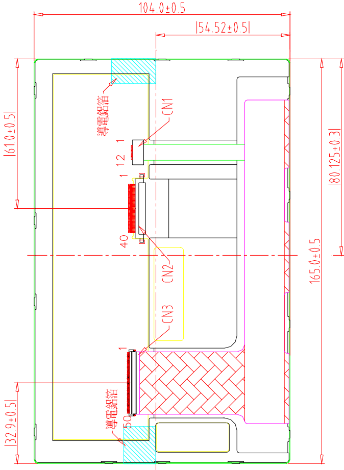
Back View
