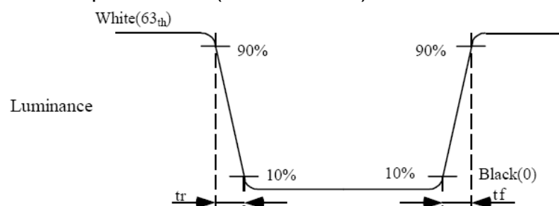
Fig9-3 Definition of Response Time(White-Black)
