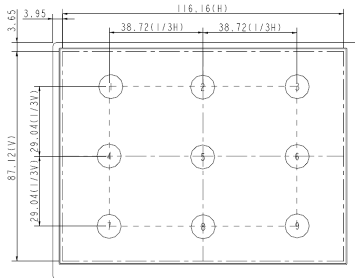
Fig9-1 Measuring point
