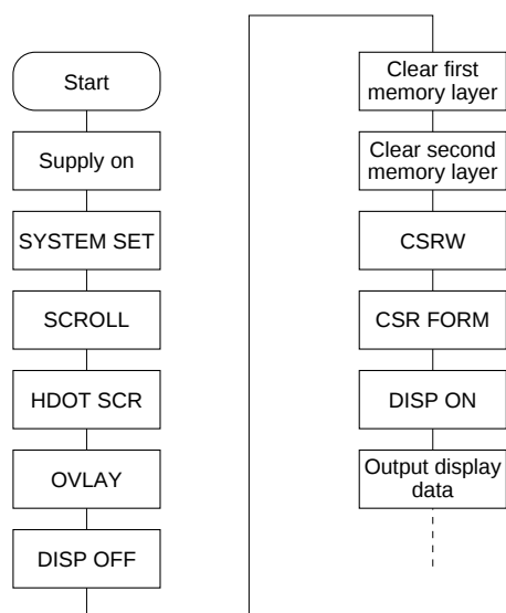
Figure 57. Initialization procedure
