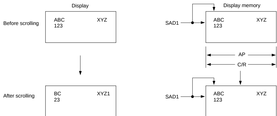
Figure 42. Horizontal wraparound scrolling
