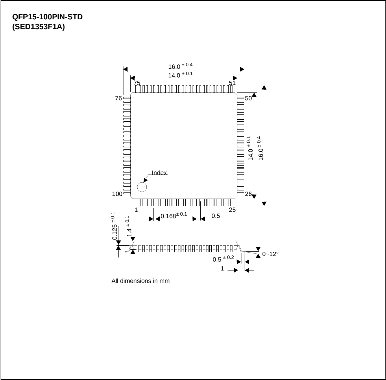
Figure 51: Mechanical Drawing QFP15-100-STD (SED1353F1A)
