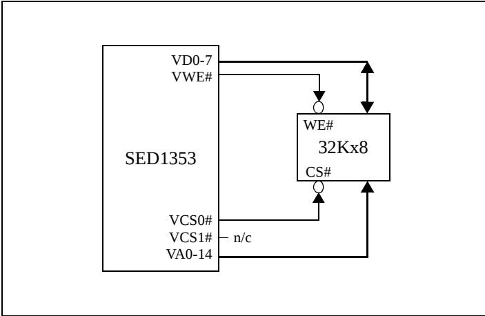
Figure 44: 8-Bit Mode - 32K bytes SRAM (Requires AUX[01] bit 0 = 1)
